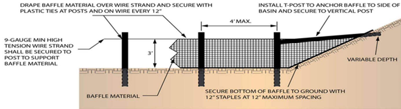
SIDE VIEW
